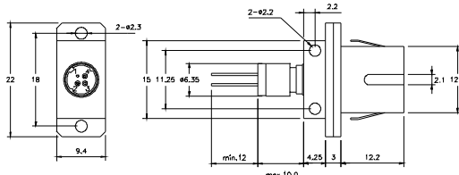
SC Receptacle (Board Mount)
